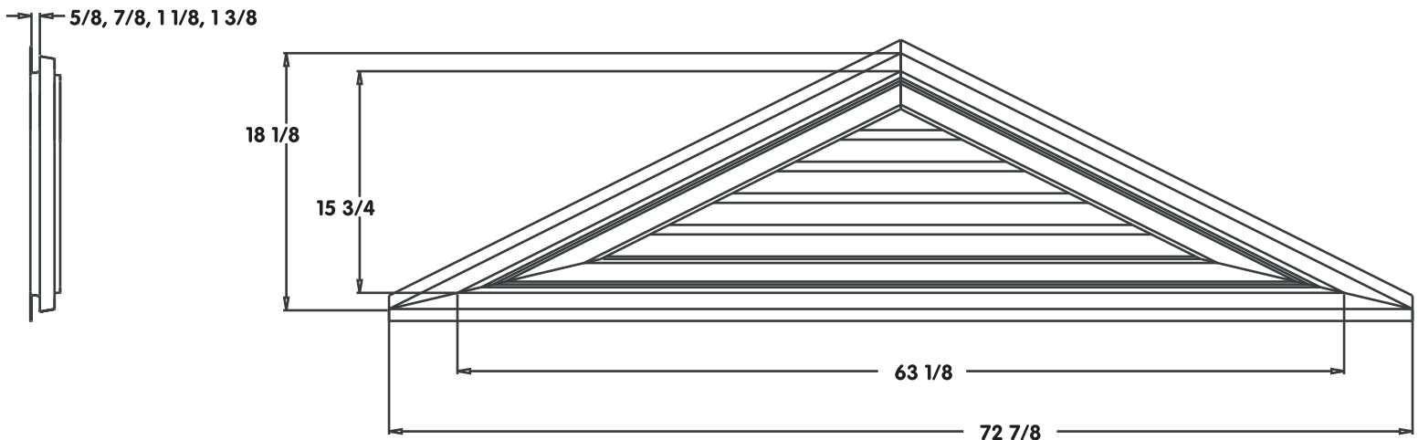
18 X 72.5 6/12 PITCH NOTE: ACTUAL DIMENSIONS MAY VARY SLIGHTLY
